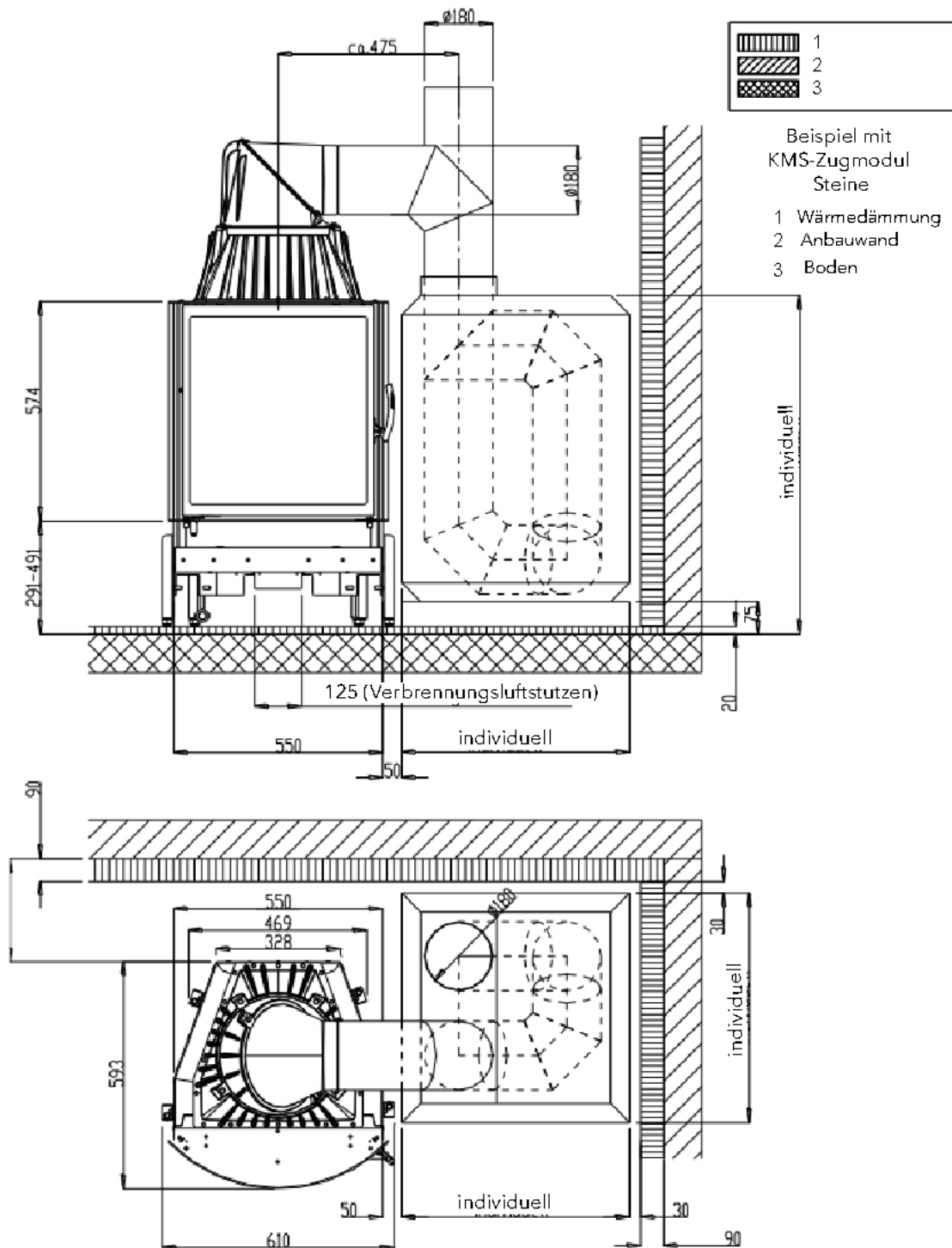
Abb. 14: KMS System
