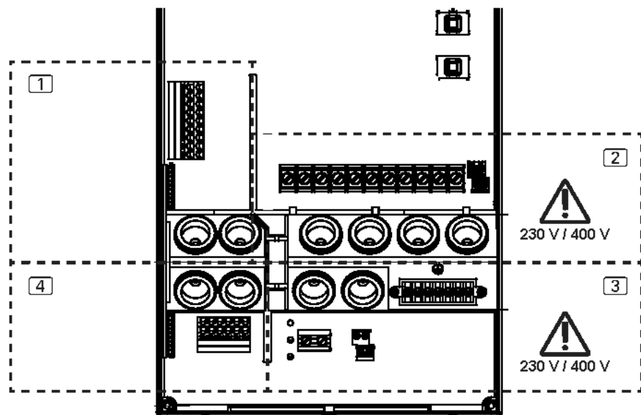
Fig. 4 Connection areas
