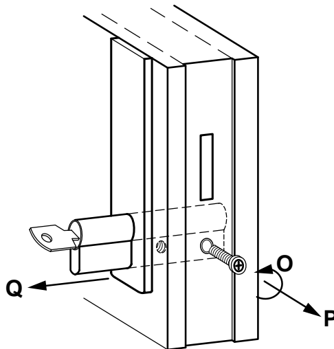
Fig. 4: Replacing the lock cylinder
