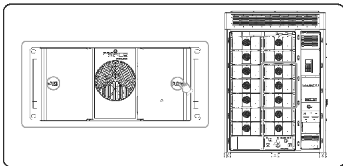
Figure 6-2 Opening the battery pack cover
