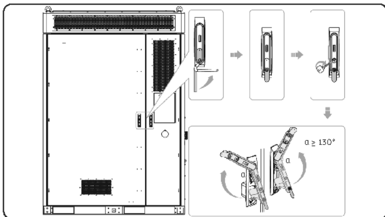
Figure 2-4 Opening front doors
