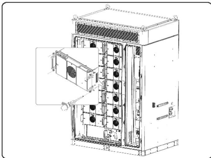
Figure 6-5 Removing screws on the battery pack
