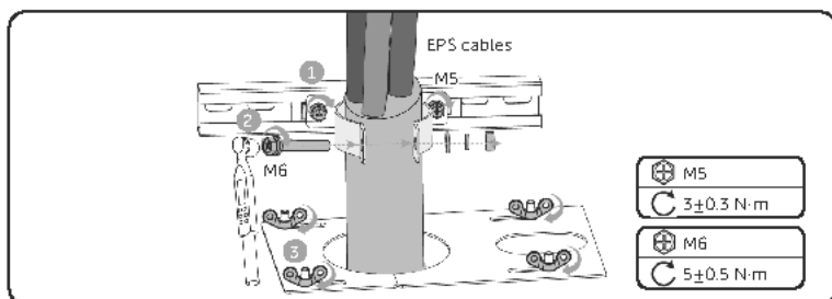
Figure 21-16 Tightening screws
