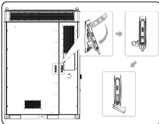
Figure 13-8 Closing the door
