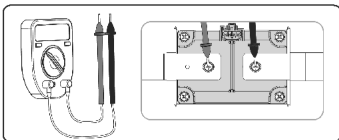
Figure 12-8 Measuring the contactor ON-OFF status
