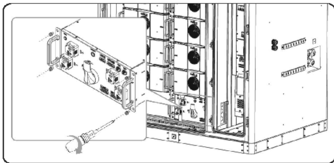
Figure 11-6 Removing screws on high-voltage box
