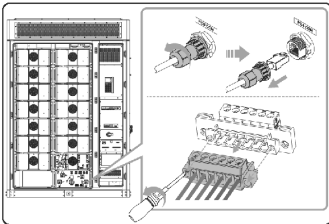
Figure 11-5 Removing cables of high-voltage box
