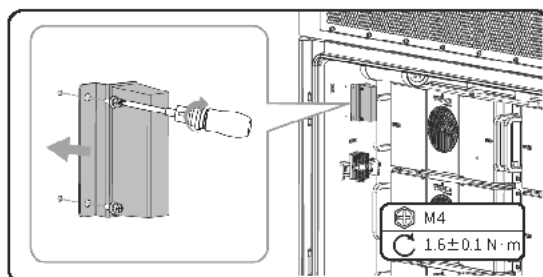
Figure 24-5 Installing the CO detector
