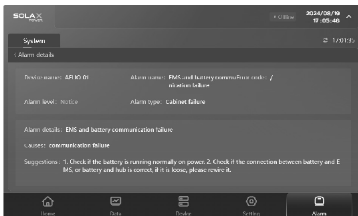
Figure 3-4 Alarm details
