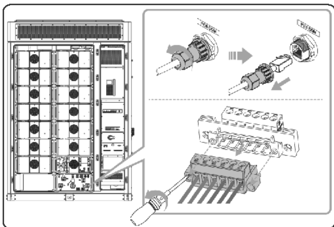
Figure 10-5 Removing cables of high-voltage box
