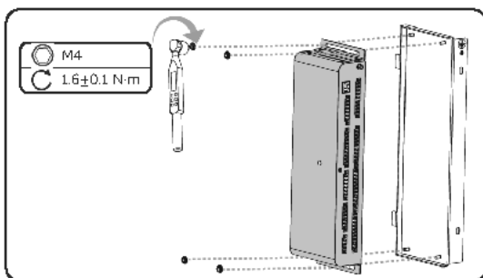
Figure 15-5 Assembling IO modules and brackets
