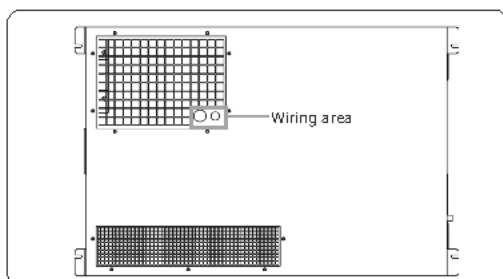
Figure 17-2 Removing cables (top view)
