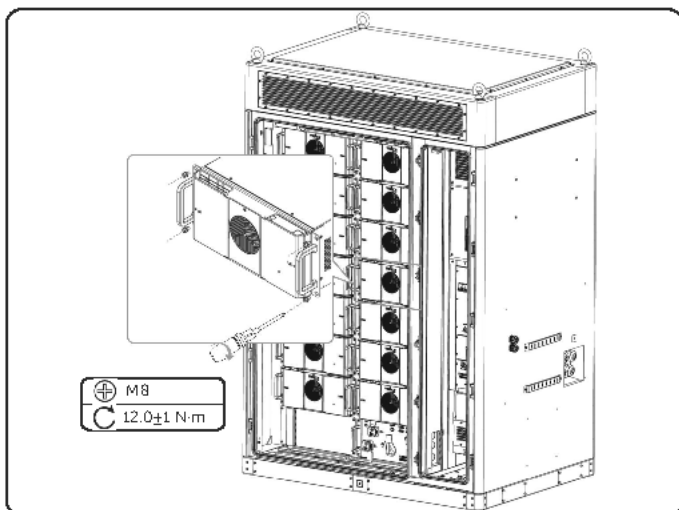
Figure 6-6 Installing the battery pack
