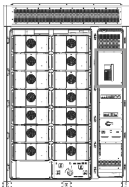
Figure 15-1 Position of the I/O module
