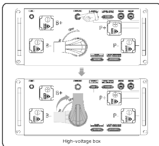
Figure 2-6 Shutting down the high-voltage box
