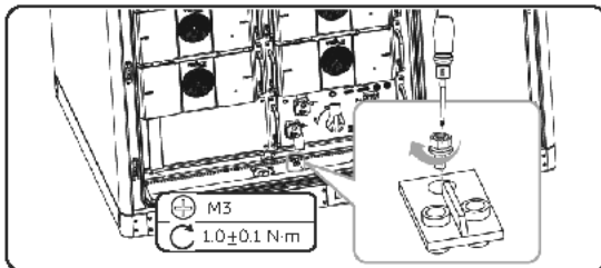
Figure 25-4 Installing the water sensor
