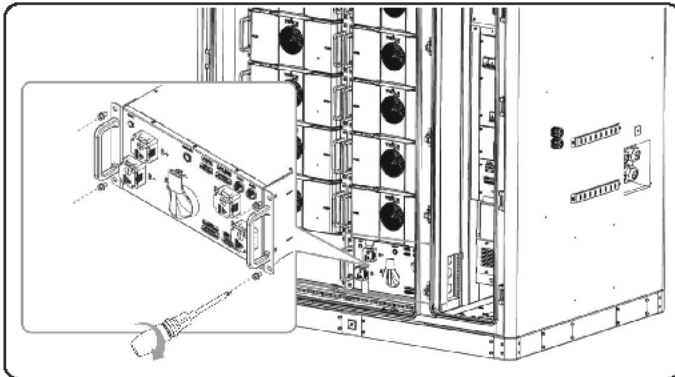
Figure 9-6 Removing screws on high-voltage box
