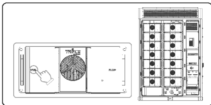
Figure 10-2 Opening the battery pack cover
