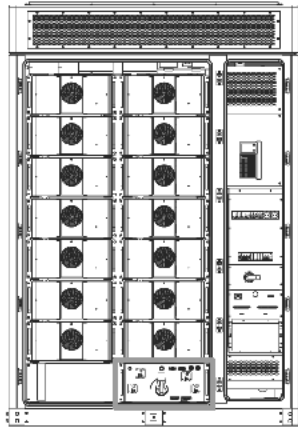
Figure 9-1 Position of the high-voltage box
