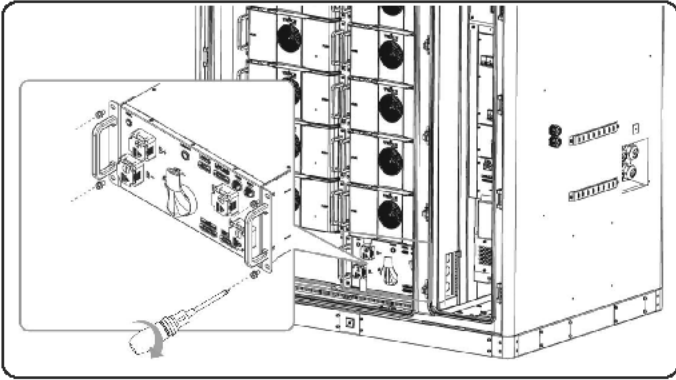
Figure 12-6 Removing screws on high-voltage box
