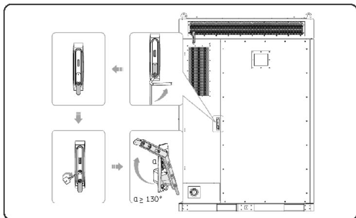
Figure 13-2 Opening rear door
