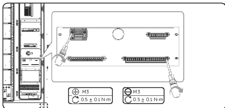
Figure 21-26 Connecting the cables
