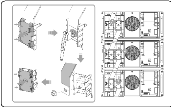
Figure 6-3 Removing the copper bars
