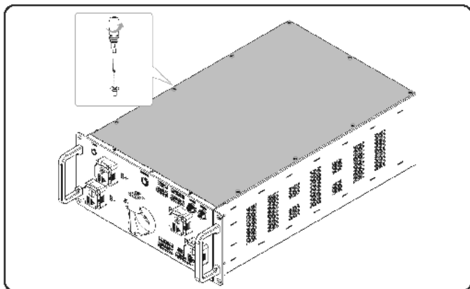
Figure 11-7 Removing the top cover
