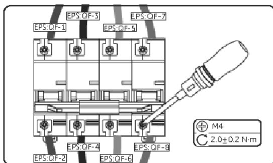
Figure 26-6 Connecting EPS switch cables
