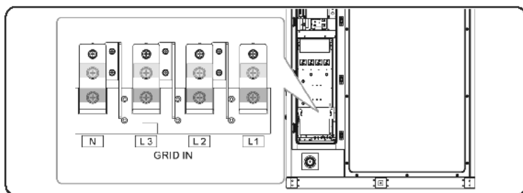
Figure 21-21 Connection area
