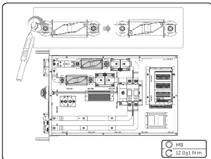
Figure 12-12 Installing the fuses (top view)
