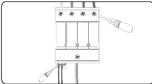
Figure 22-3 Removing the SPD module
