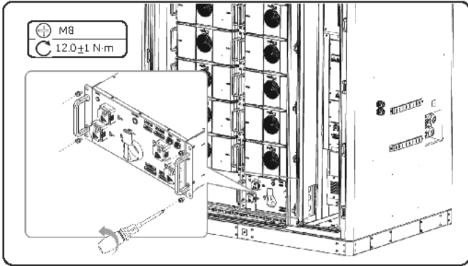
Figure 9-7 Installing the high-voltage box
