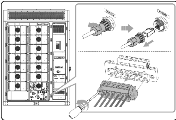
Figure 12-5 Removing cables of high-voltage box
