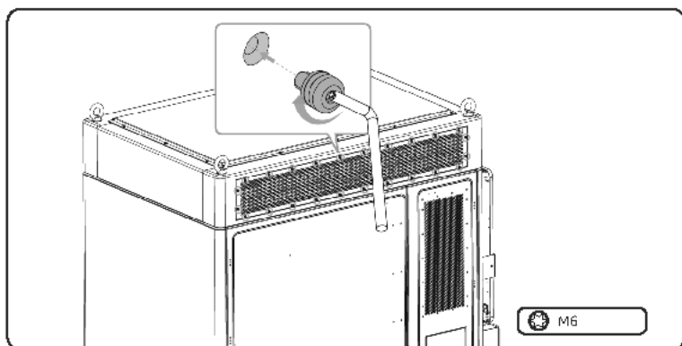
Figure 4-12 Tightening M6 screws
