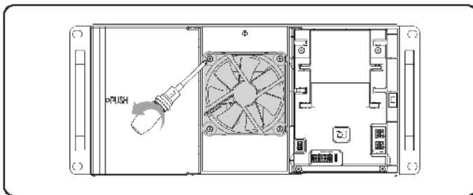
Figure 7-5 Removing the fan
