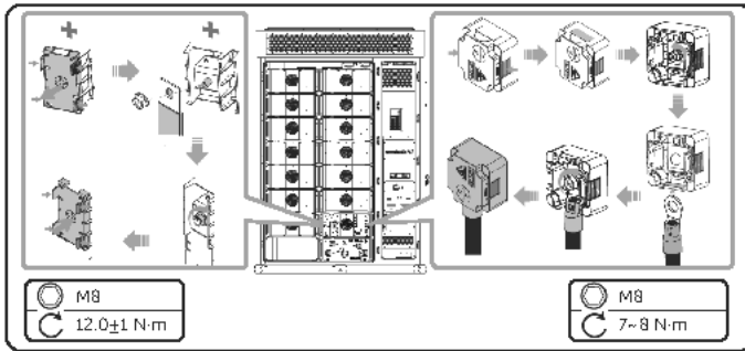
Figure 9-9 Connecting the copper bars and cables
