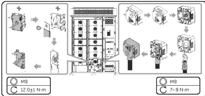
Figure 12-17 Connecting the copper bars and cables
