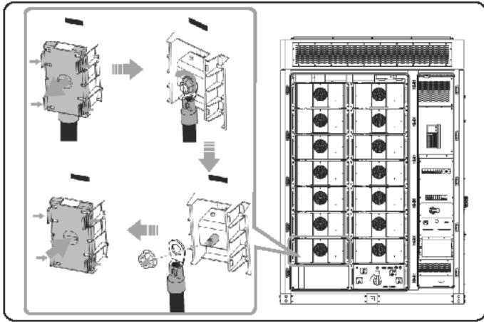
Figure 9-3 Removing the negative power cable
