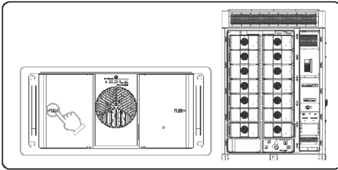
Figure 9-11 Closing the battery pack covers
