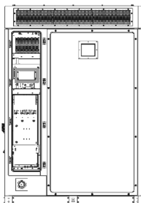
Figure 13-1 Position of the EMS1000 (rear view)
