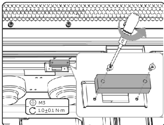
Figure 19-4 Installing the door sensor
