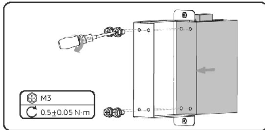
Figure 14-6 Installing the new Switch
