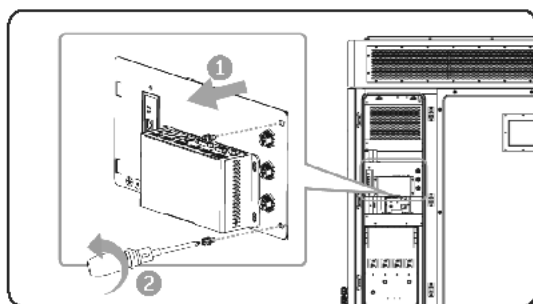
Figure 14-3 Removing the sheet metal
