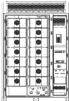
Figure 12-1 Position of the high-voltage box contactors
