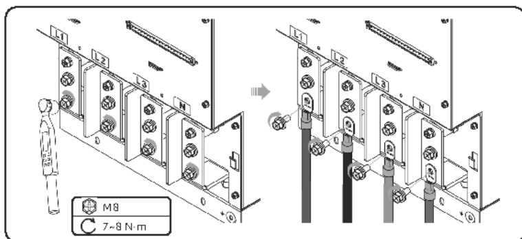
Figure 21-15 Connecting L1, L2, L3 and N cables
