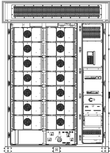
Figure 17-1 Position of the air conditioner
