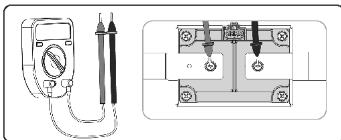
Figure 12-13 Measuring the contactor ON-OFF status
