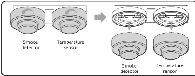
Figure 20-2 Removing the smoke detector and temperature sensor
