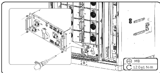
Figure 11-13 Installing the high-voltage box
