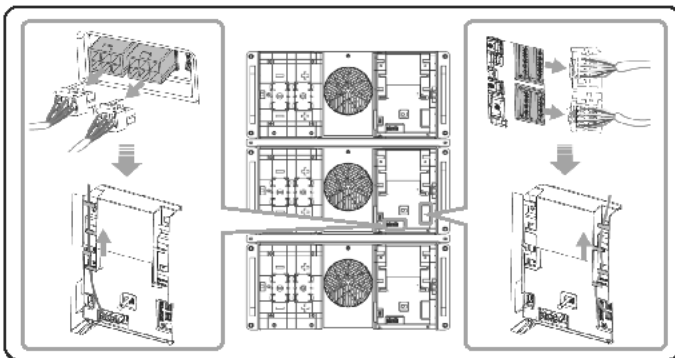
Figure 6-4 Removing the cables
