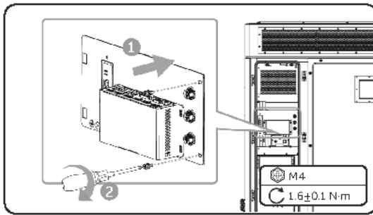
Figure 13-7 Installing the sheet metal
