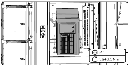
Figure 16-4 Installing the UPS
