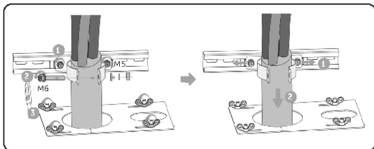
Figure 21-3 Removing the EPS cables
