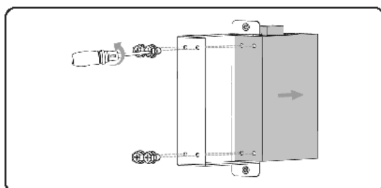
Figure 14-5 Removing the Switch
