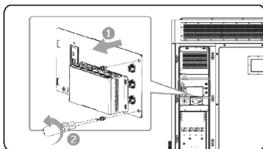
Figure 13-4 Removing the sheet metal
