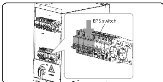
Figure 26-5 Installing the EPS switch
