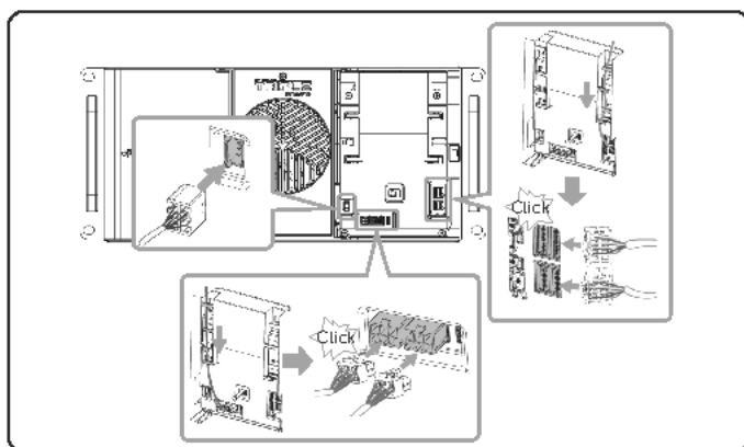
Figure 8-10 Connecting the cables of battery pack
