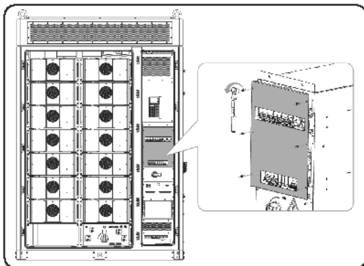
Figure 26-2 Removing the front panel
