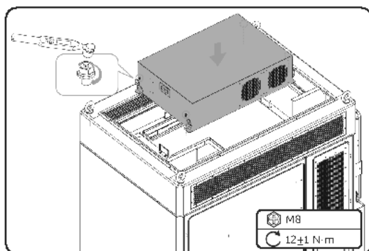
Figure 17-4 Installing the new air conditioner
