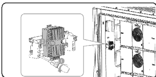
Figure 18-2 Removing temperature and humidity sensor
