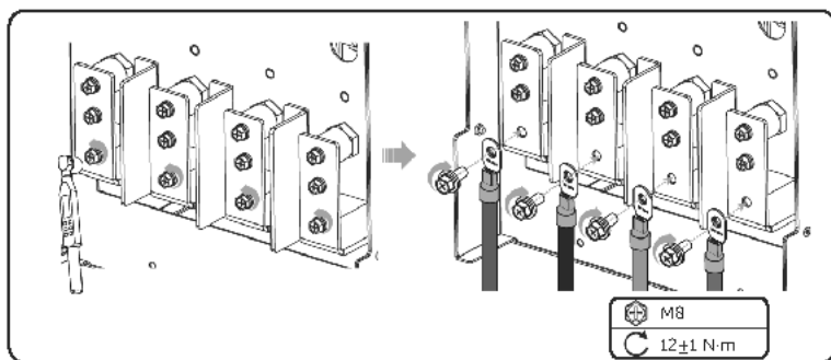
Figure 21-22 Connecting L1, L2, L3 and N cables
