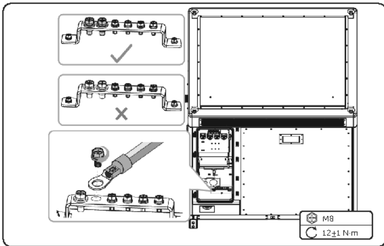
Figure 21-24 Connecting PE wire
