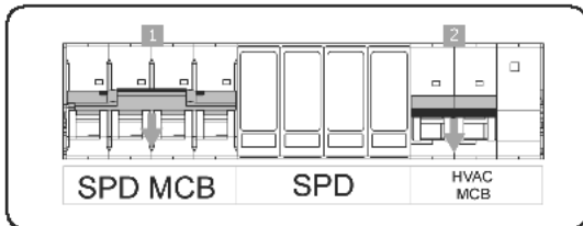
Figure 2-8 Flipping down breakers
