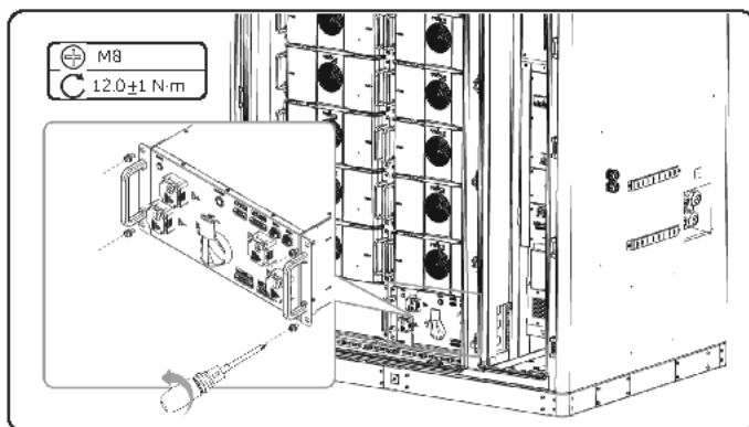
Figure 12-15 Installing the high-voltage box
