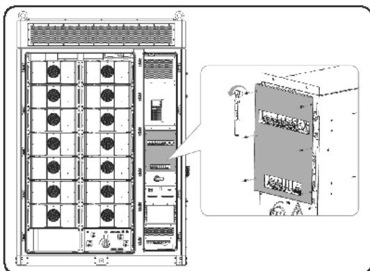
Figure 27-2 Removing the front panel
