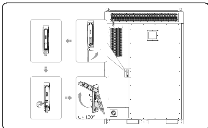
Figure 21-6 Opening rear door
