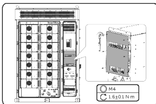
Figure 26-7 Mounting the panel
