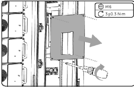
Figure 16-5 Mounting the panel
