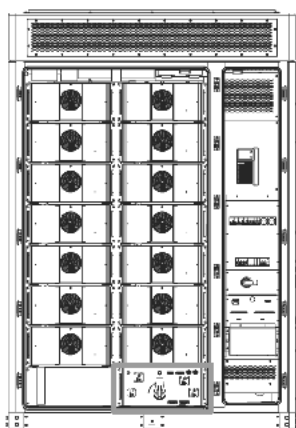
Figure 10-1 Position of the SBMU
