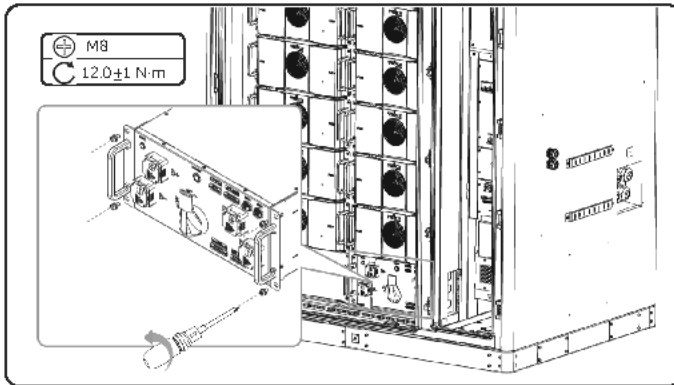
Figure 10-11 Installing the high-voltage box
