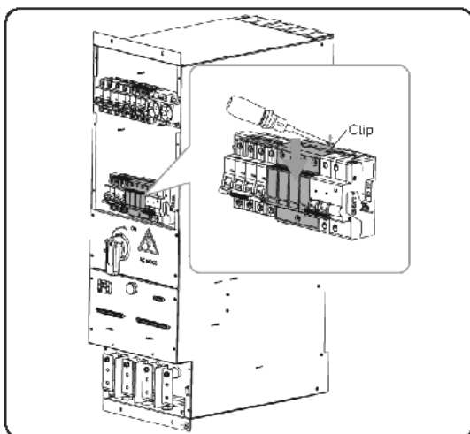
Figure 22-5 Installing the SPD module
