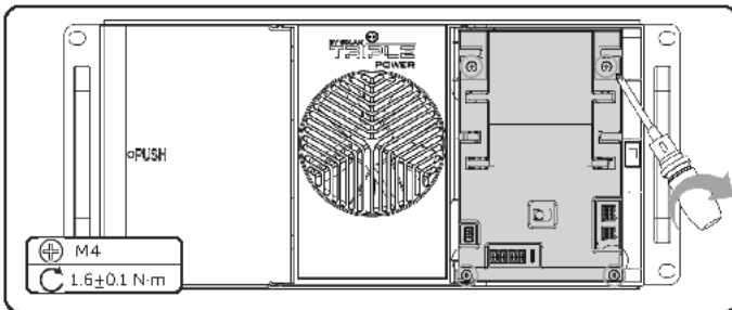
Figure 8-9 Installing the PCBA cover
