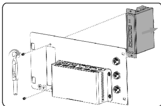
Figure 14-4 Removing the Switch from the sheet metal
