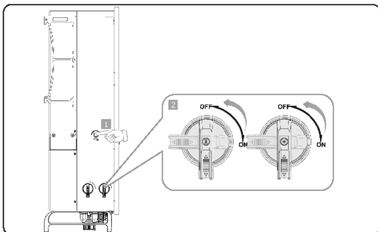
Figure 2-5 Shutting down the inverter
