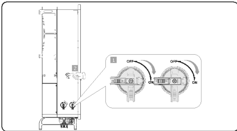
Figure 2-18 Starting the inverter
