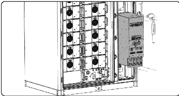
Figure 21-10 Removing distribution box
