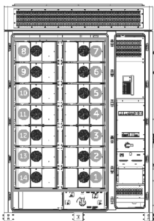
Figure 6-1 Position of the battery packs
