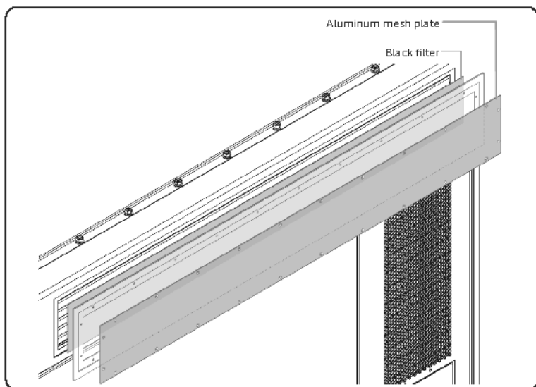
Figure 4-11 Dismantling aluminum mesh plate and black filter
