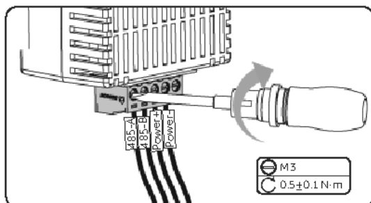
Figure 18-4 Connecting the cables
