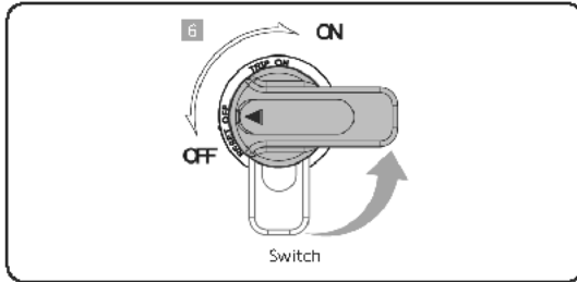
Figure 2-10 Rotating switch
