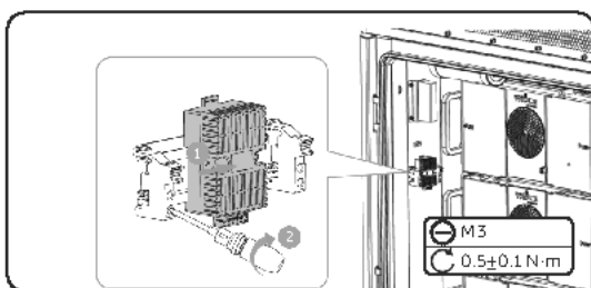
Figure 18-3 Installing temperature and humidity sensor
