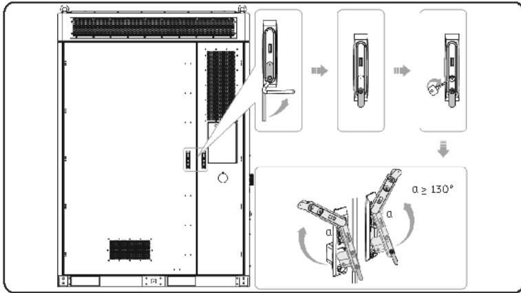
Figure 2-1 Opening front doors
