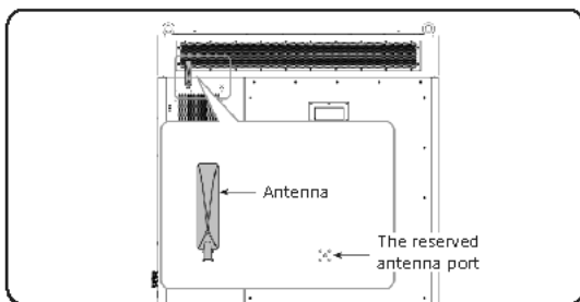
Figure 5-5 Well installed antenna
