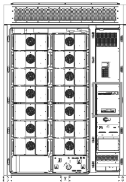
Figure 27-1 Position of UPS switch
