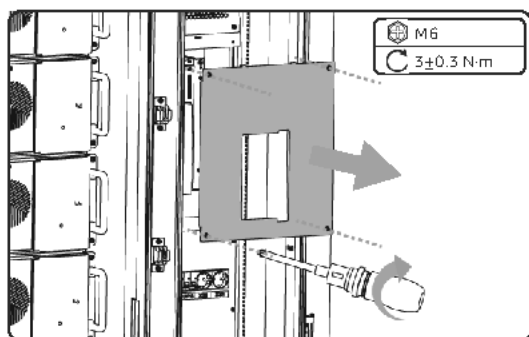
Figure 15-7 Mounting the panel
