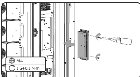
Figure 15-6 Installing IO modules
