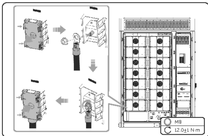
Figure 10-12 Connecting the negative power cable
