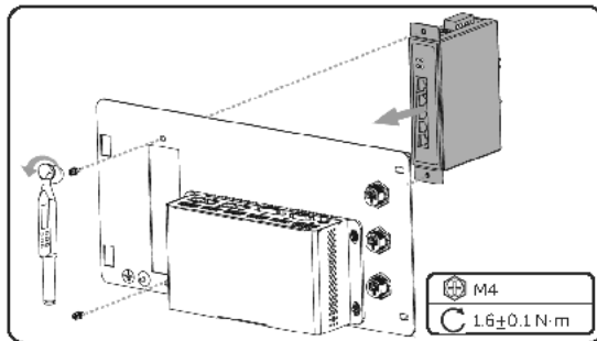
Figure 14-7 Installing the Switch
