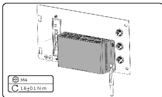
Figure 13-6 Installing a new EMS1000
