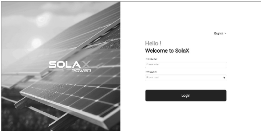
Figure 3-5 Login page
