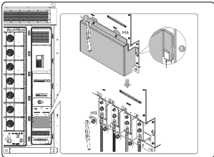
Figure 21-2 Disconnecting EPS cables
