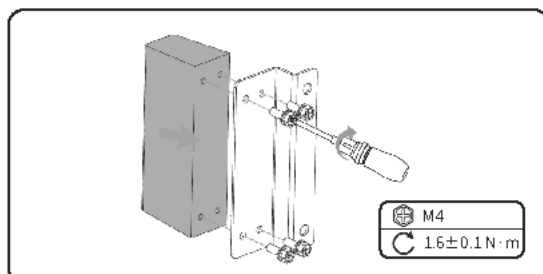
Figure 24-4 Installing the CO detector
