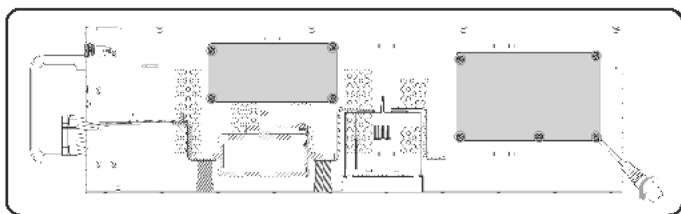
Figure 10-8 Removing the SBMU (right view)
