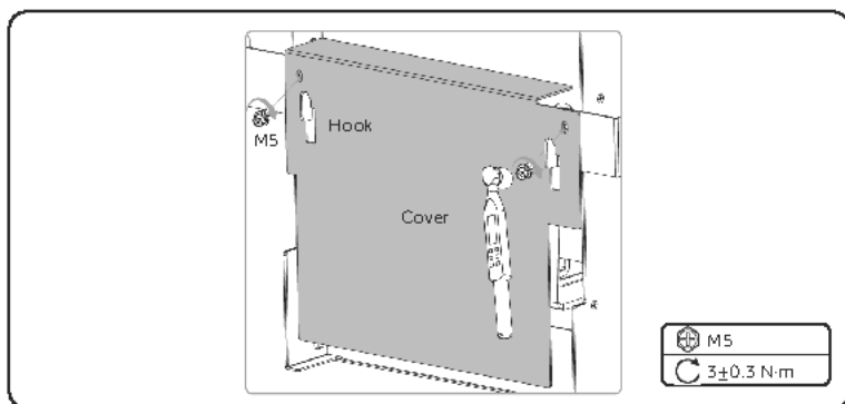
Figure 21-25 Reattaching cover
