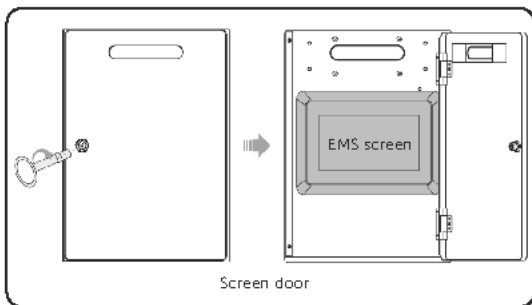
Figure 3-1 Unlocking screen door
