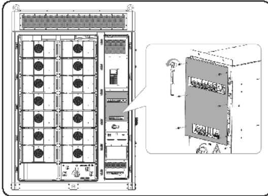
Figure 22-2 Removing the front panel
