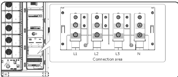
Figure 21-14 Connection area
