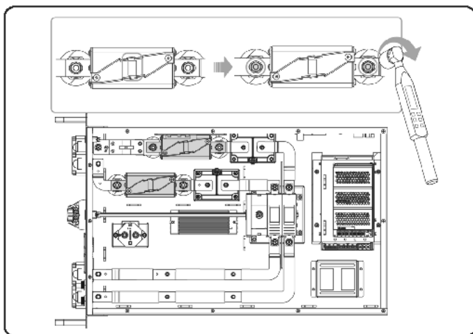
Figure 12-9 Removing the fuses (top view)
