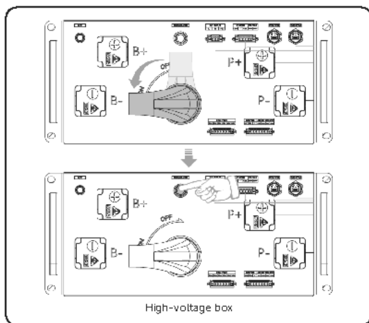
Figure 2-20 Starting the high-voltage box
