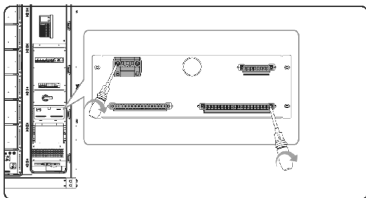
Figure 21-5 Removing the terminals
