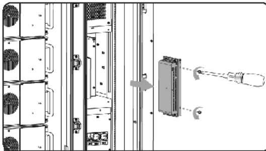
Figure 15-3 Removing the IO module
