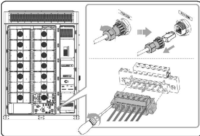
Figure 9-5 Removing cables of high-voltage box
