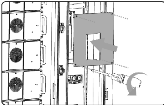
Figure 16-1 Removing the panel
