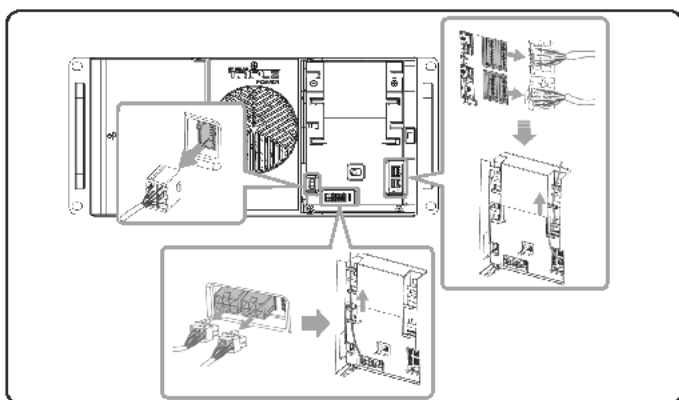
Figure 8-3 Removing the cables
