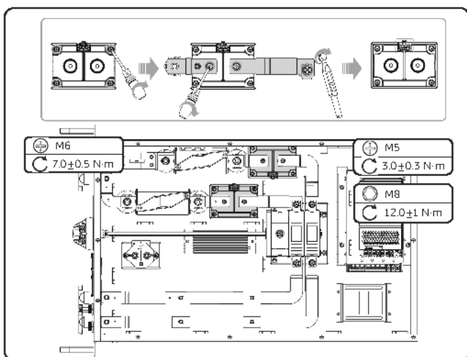
Figure 12-11 Installing the contactors (top view)
