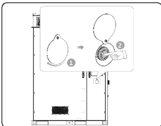
Figure 2-13 Pressing emergency stop button
