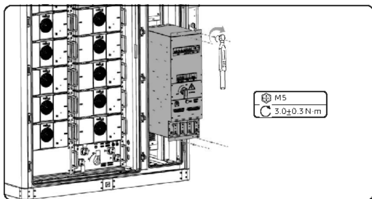
Figure 21-11 Installation of distribution box
