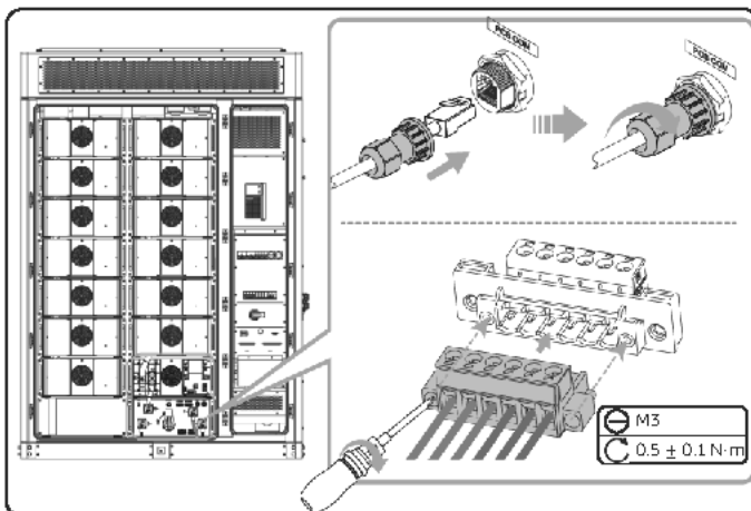
Figure 9-10 Connecting cables of high-voltage box
