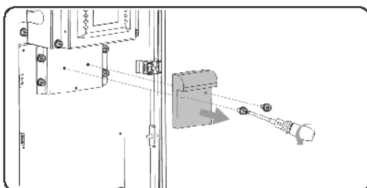
Figure 23-2 Removing audible and visual alarm
