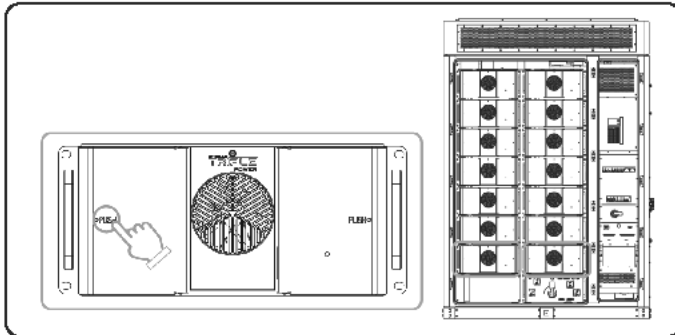
Figure 9-2 Opening the battery pack cover
