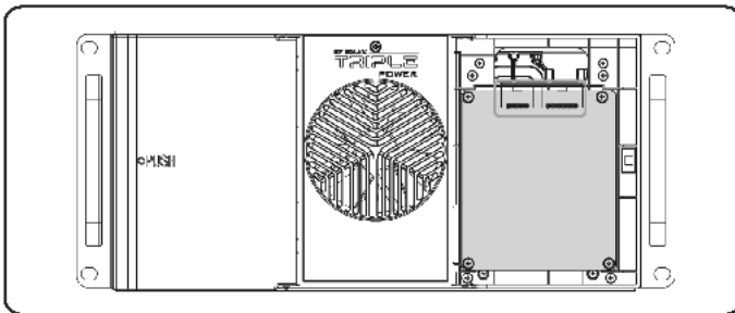
Figure 8-8 Connecting the cables of the BMU
