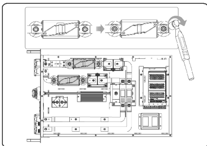
Figure 11-9 Removing the fuses (top view)
