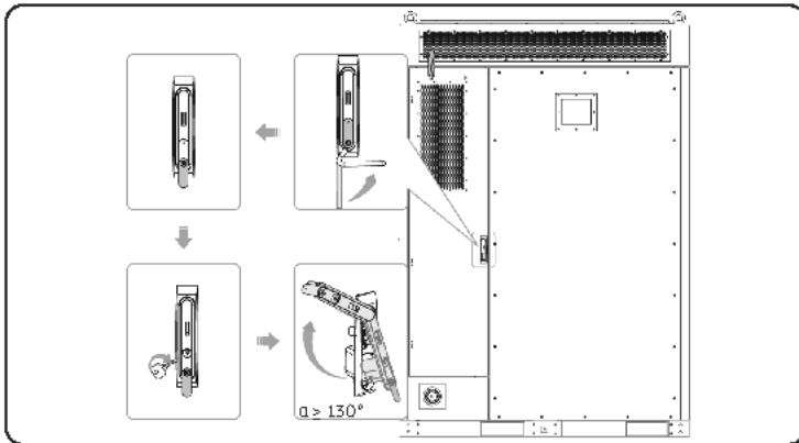
Figure 14-2 Opening the rear door
