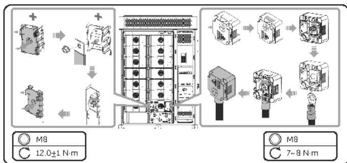
Figure 10-13 Connecting the copper bars and cables
