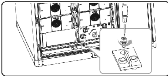
Figure 25-3 Removing the water sensor
