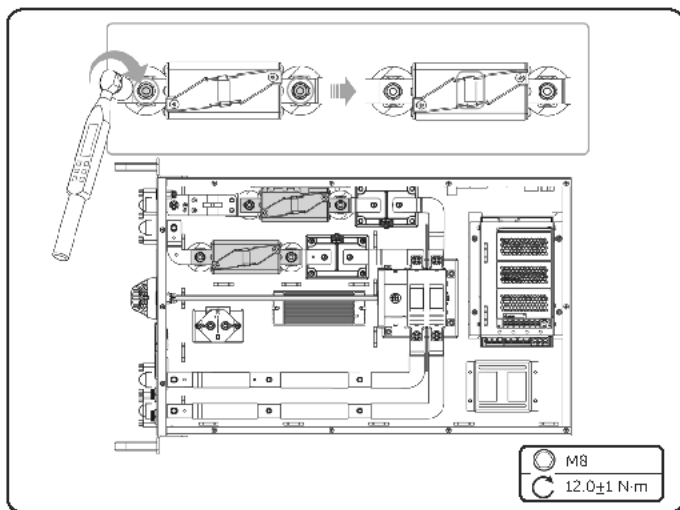
Figure 11-10 Installing the fuses (top view)
