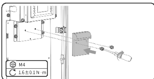
Figure 23-3 Installation of audible and visual alarm
