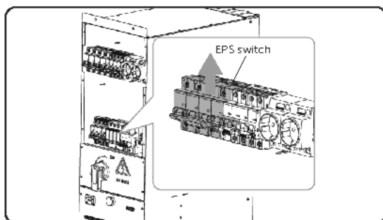
Figure 26-4 Removing the EPS switch
