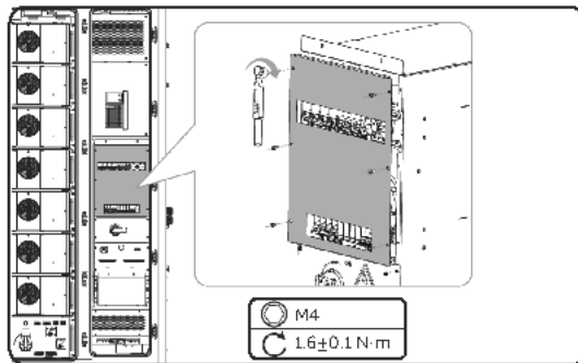
Figure 27-7 Mounting the panel
