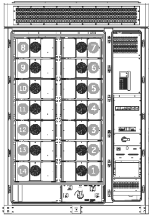
Figure 7-1 Position of the battery pack fans
