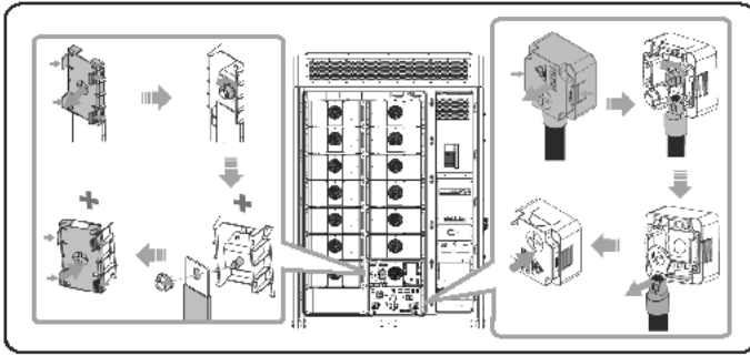
Figure 12-4 Removing the copper bars and cables
