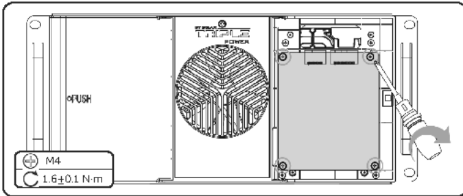
Figure 8-7 Installing a new BMU
