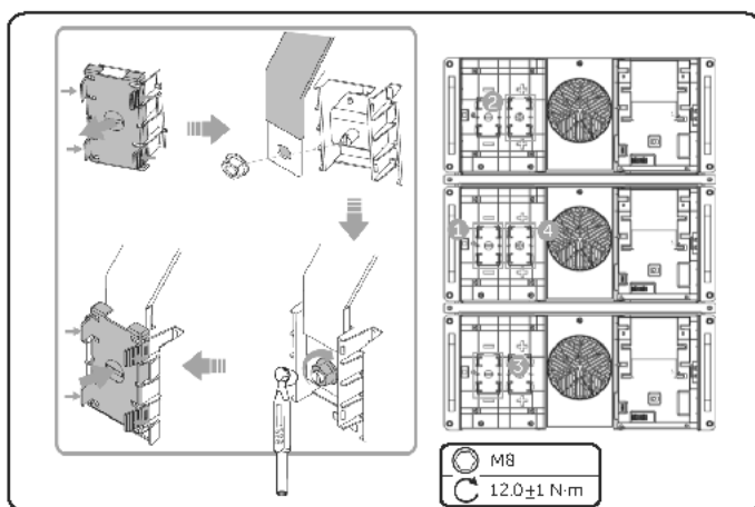
Figure 6-7 Installing the copper bars
