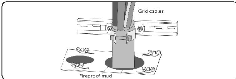
Figure 21-28 Plugging the cables threading hole on the rear side
