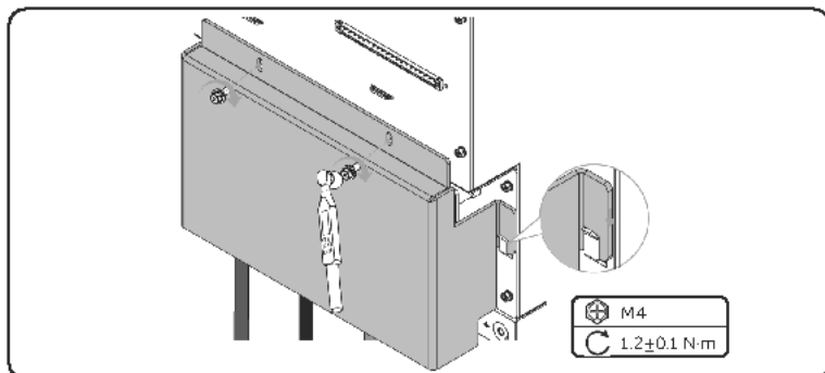
Figure 21-17 Securing cover
