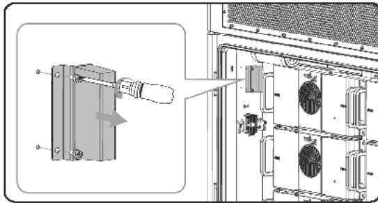
Figure 24-2 Removing the CO detector
