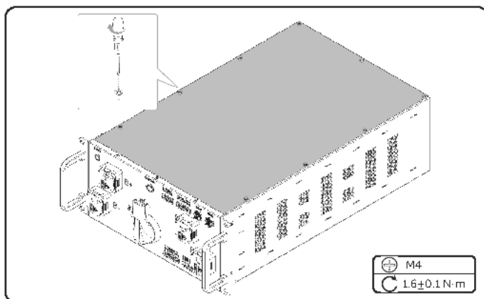
Figure 12-14 Installing the top cover
