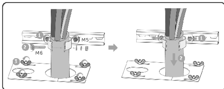
Figure 21-8 Removing the Grid cables
