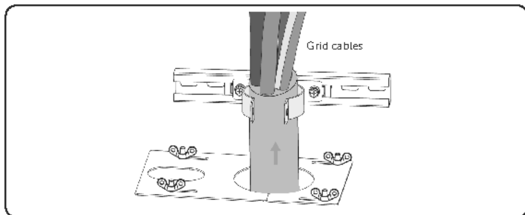
Figure 21-20 Threading grid cables
