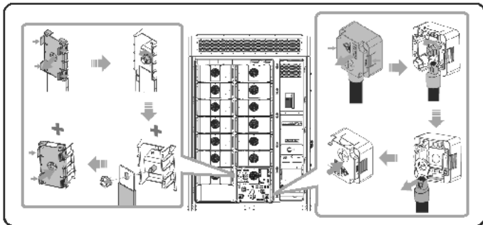
Figure 9-4 Removing the copper bars and cables
