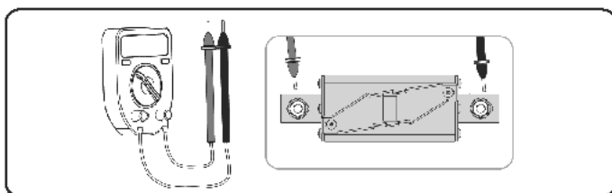
Figure 11-11 Measuring the fuse ON-OFF status
