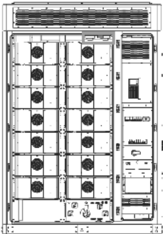
Figure 20-1 Position of the smoke detector and temperature sensor
