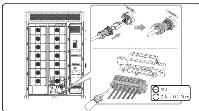
Figure 12-18 Connecting cables of high-voltage box
