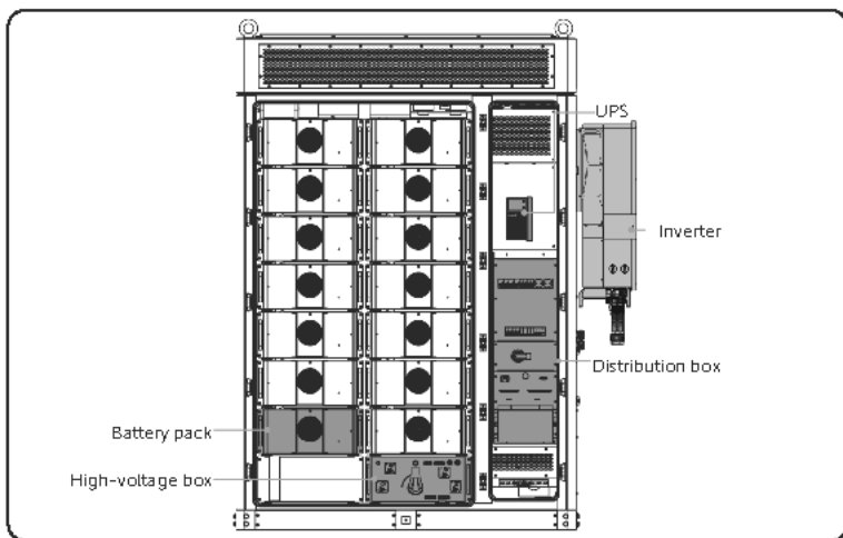
Figure 2-3 Location of modules
