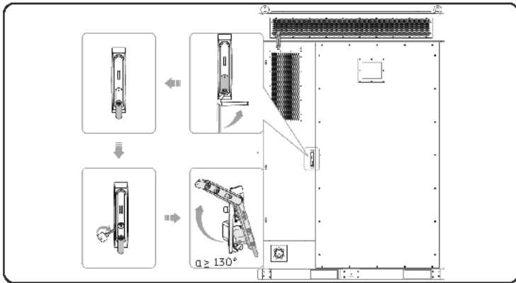
Figure 21-18 Opening rear door
