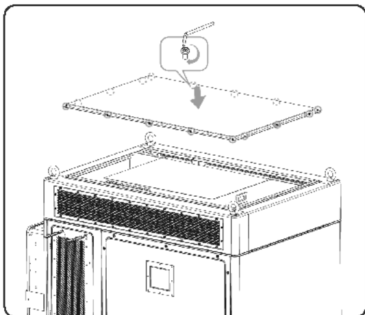
Figure 17-5 Installing top cover
