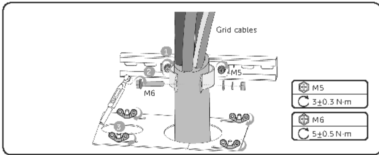
Figure 21-23 Tightening screws
