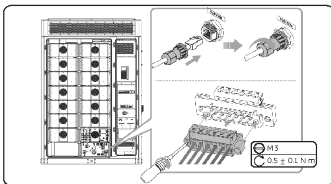
Figure 10-14 Connecting cables of high-voltage box
