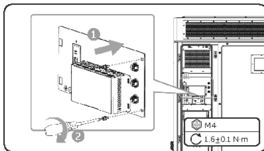
Figure 14-8 Installing the sheet metal
