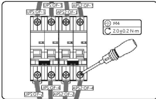
Figure 27-6 Connecting UPS switch cables
