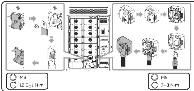
Figure 11-15 Connecting the copper bars and cables
