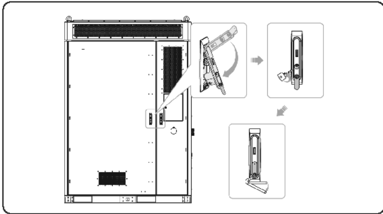
Figure 2-21 Closing the door
