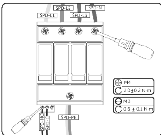
Figure 22-6 Connecting the SPD module cables
