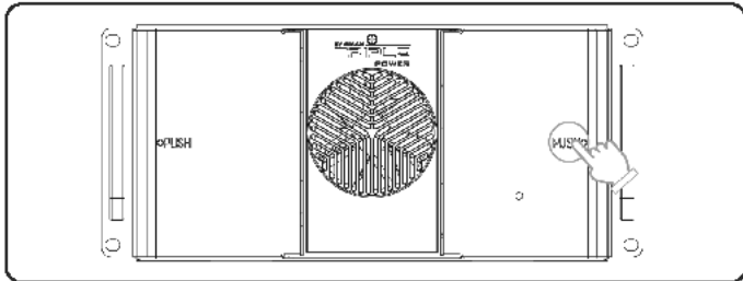
Figure 7-2 Opening the battery pack cover
