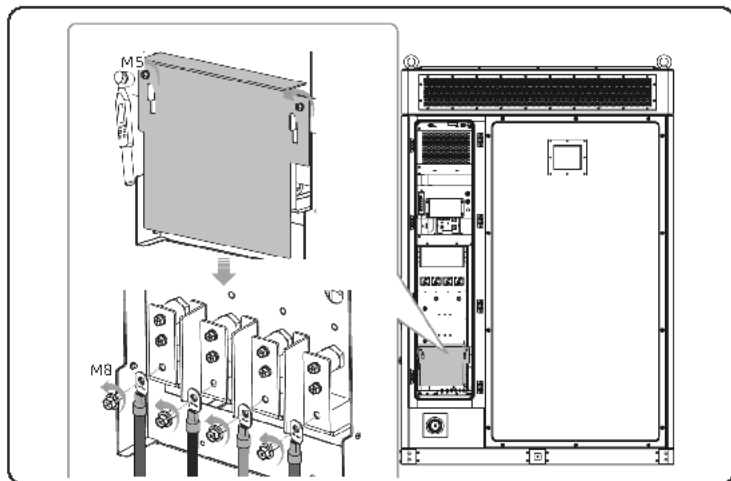
Figure 21-7 Disconnecting Grid cable
