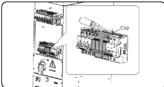
Figure 22-4 Removing the SPD module
