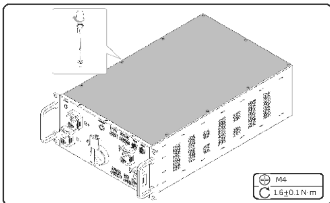
Figure 11-12 Installing the top cover
