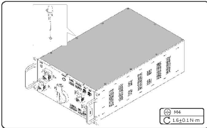
Figure 10-10 Installing the top cover
