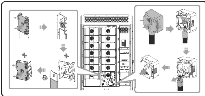
Figure 10-4 Removing the copper bars and cables
