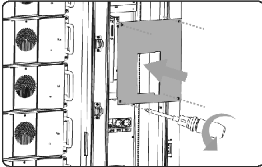
Figure 15-1 Removing panel
