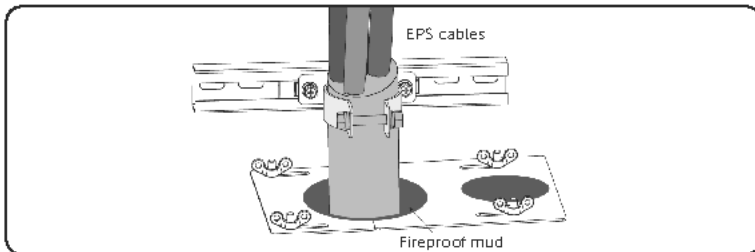
Figure 21-27 Plugging the cables threading hole on the front side
