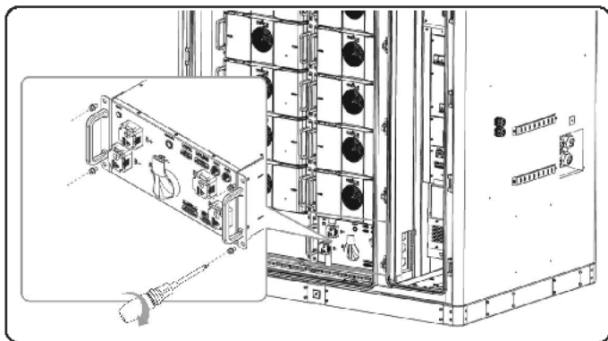
Figure 10-6 Removing screws on high-voltage box
