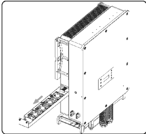
Figure 28-3 Pulling put the whole fan bracket
