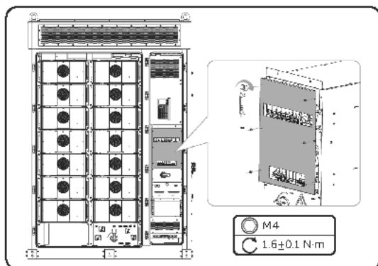
Figure 22-7 Mounting the panel
