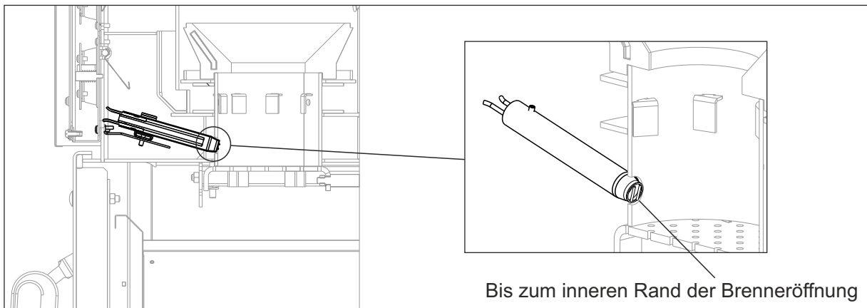
Detail D
